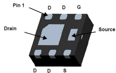
DFN2X2-6L (thickness 0.5cm)
